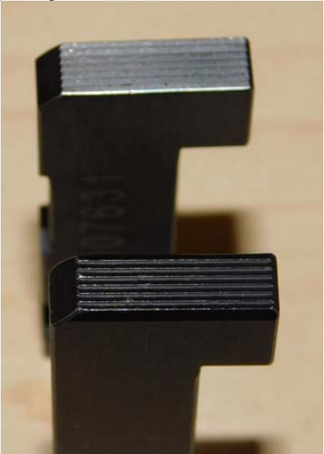
ES-007631 Cable gripping jaws Soft version Grip lining with deburred teeth
