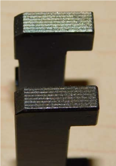
ES-007677 Cable gripping jaws, Special incl. 4 screws M3x6 diamond coated for pressure-sensitive and hard insulations
